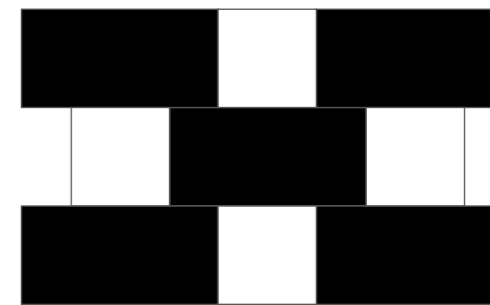
BUTTONS & BATTENS | LAYOUT 2 30x30 .12"x14" 66,67% 30x60 .12"x24" 33,33%
