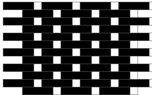
BUTTONS & BATTENS | LAYOUT 1 7,2x30 .3"x12" 80,65% 7,2x7,2 .3"x3" 19,35%
